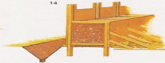
rampart excavated at the Valkenburg fort in Holland. This type of rampart was used where there was insufficient turf to face a normal rampart.
