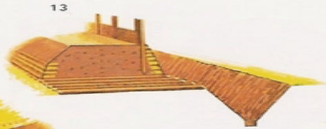
Brian Hobley. 13 Section of a turf-faced rampart built on a corduroy of logs to give it a stable foundation when the ground was soft. 14 A reconstruction of the section of the box
